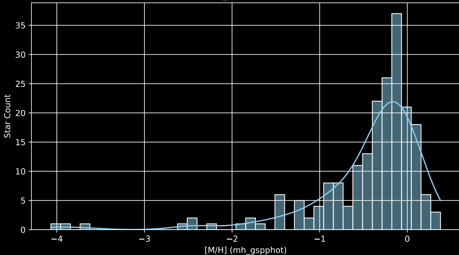
APOGEE DR17 Field: [K2_C11_001+11_btx [M/H] (mh_gspphot) (n= 205)
