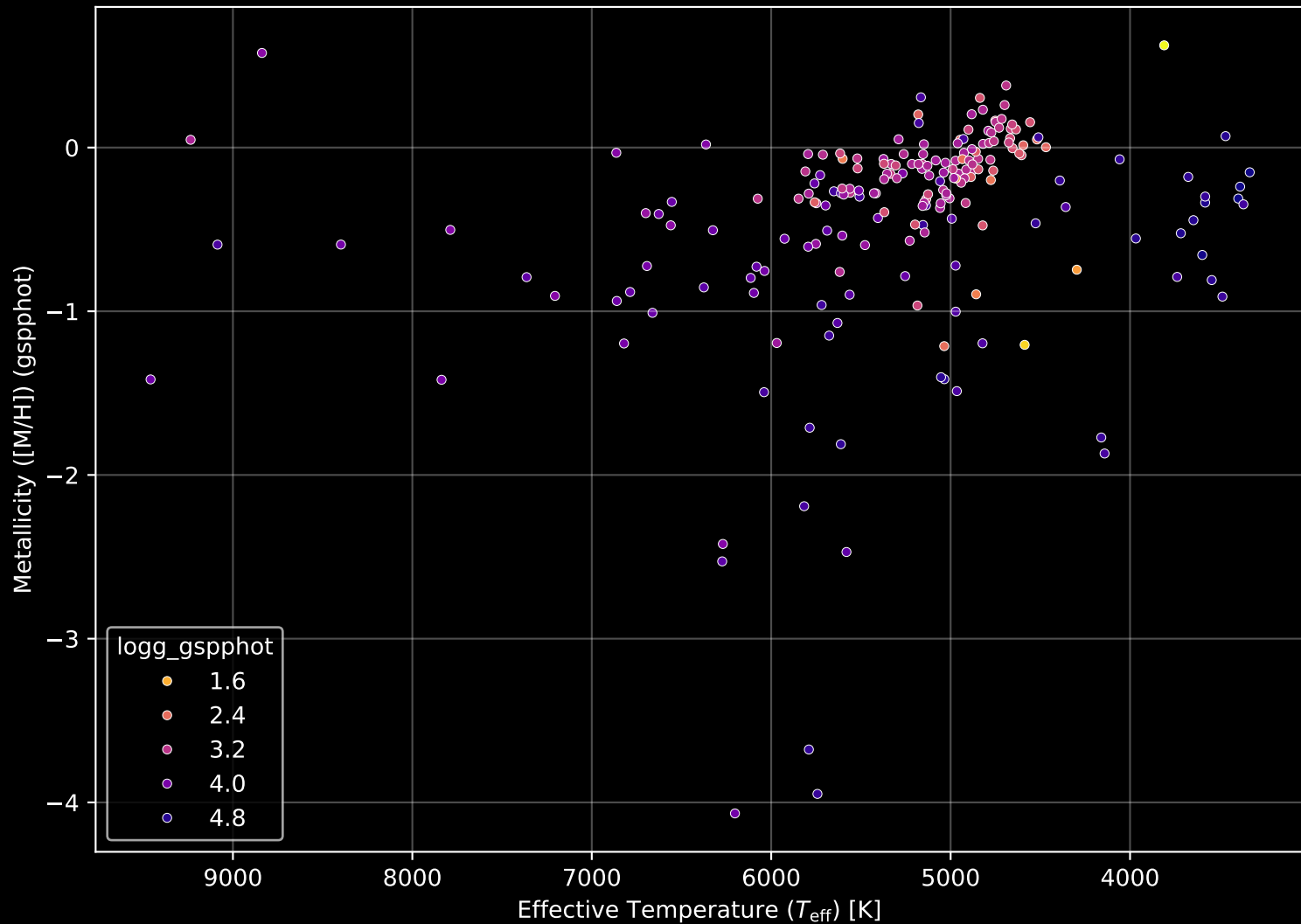
APOGEE DR17 Field: [K2_C11_001+11_btx] Stellar Population Parameters (n= 207)
