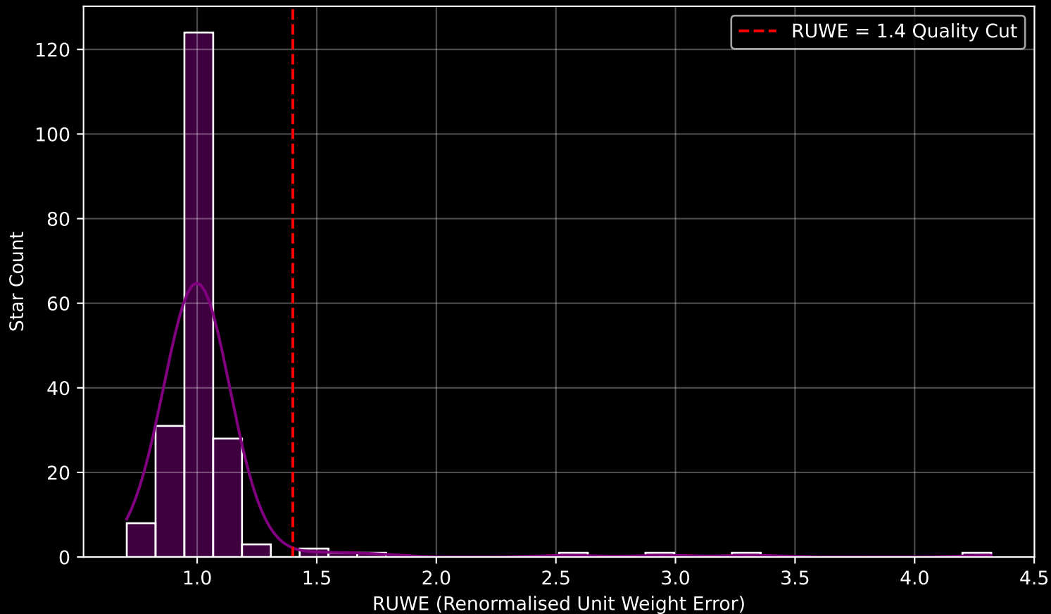
GAPOGEE DR17 Field [K2_C11_001+11_btx] RUWE Distribution (n= 202)
