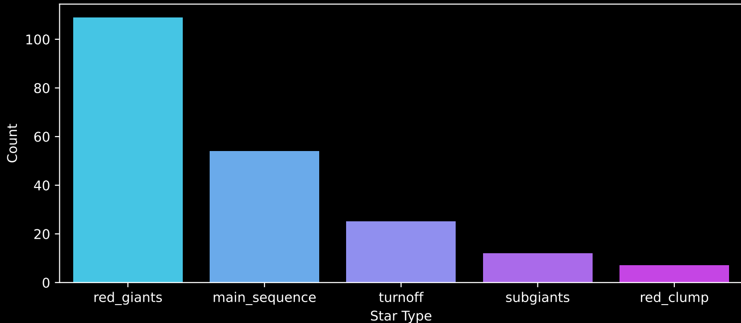
APOGEE DR17 Field: [K2_C11_001+11_btx] Count plot of Star Type
