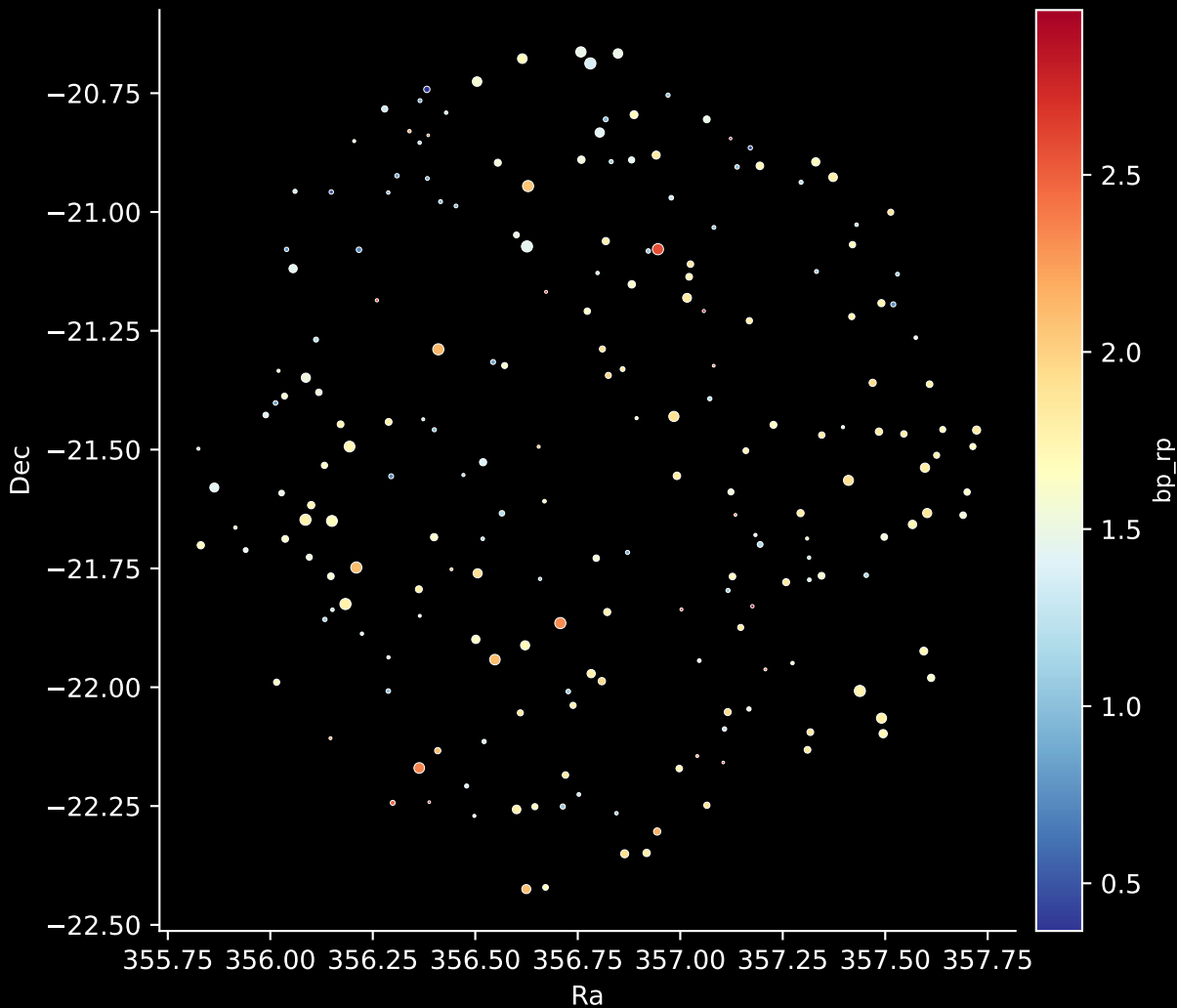
APOGEE DR17 Field: [K2_C11_001+11_btx] Stars: 207
