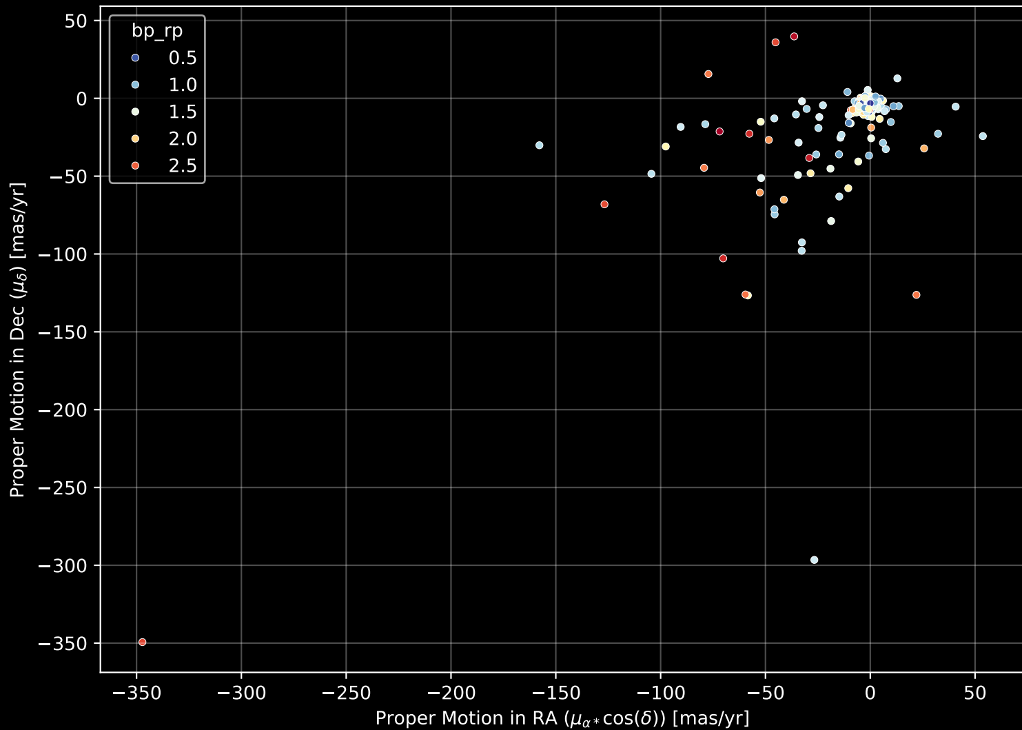
APOGEE DR17 Field: [K2_C11_001+11_btx] Proper Motion Diagram (n= 207)
