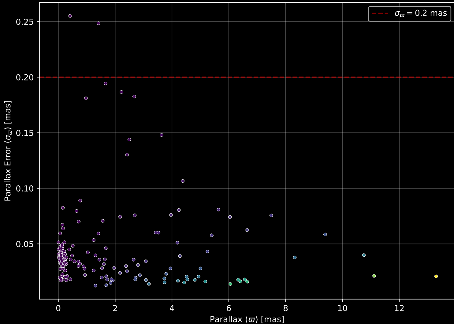
APOGEE DR17 Field: [K2_C11_001+11_btx] Parallax Quality (n= 207)
