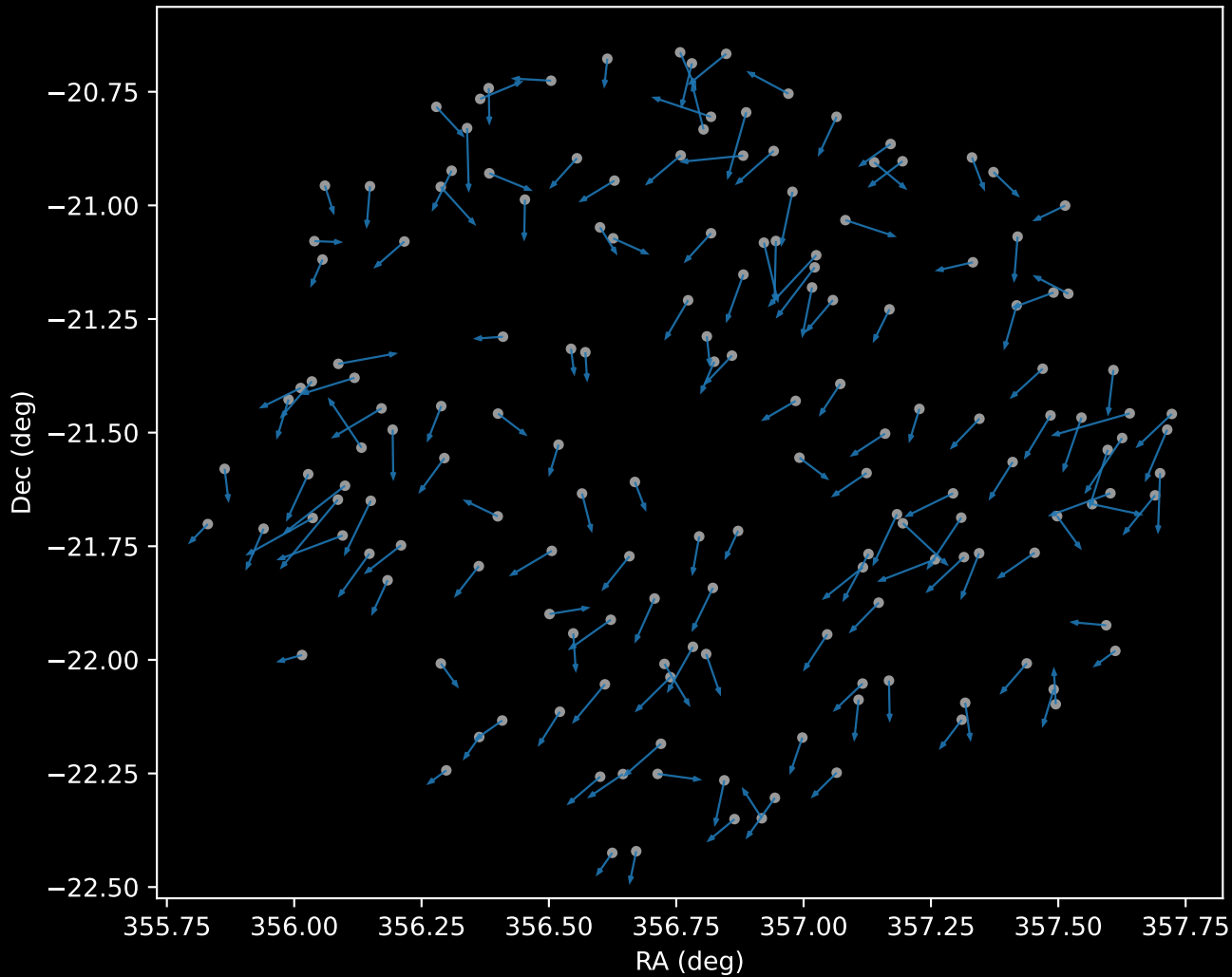
APOGEE DR17 Cluster 0 Proper Motion Vectors (n=163)
